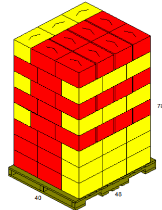
PALLET CONFIGURATION
